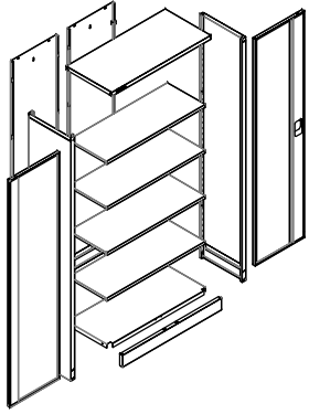
NON-ASSEMBLED VIEW
